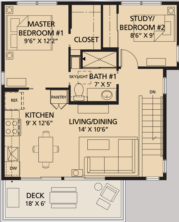
Upper Level - Cantilever
