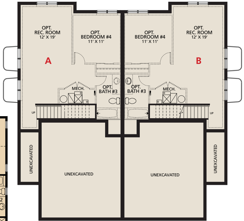
Unfinished Lower Level 8 ft 9" ceilings
