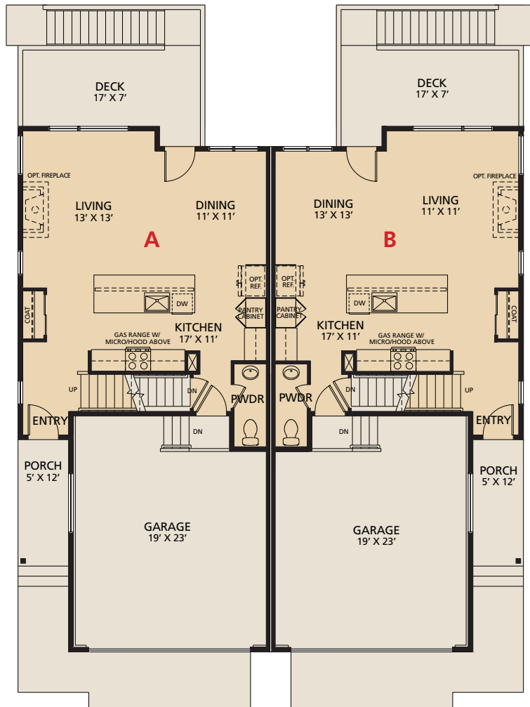
Main Level 10-ft ceilings
